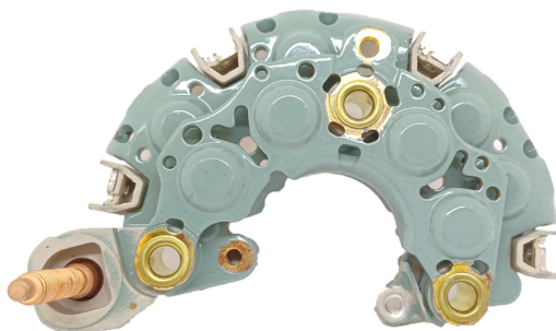
FA-N-1516 Placa Nippondenso 021580L3640, 3680, 4120, 4490, 4660, 4670, 4840, 5270. Chrysler; Dodge; Isuzu; Jeep; Toyota CON DIODO AUXILIAR
