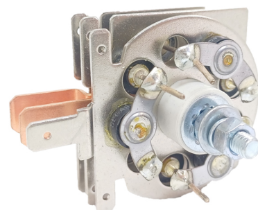
FA-L-1280 Placa Lucas 83166 /842, 84443, UBB110 Alternadores Lucas series 16ACR, 18ACR; 28-43A ER/EF, IR/EF Lotus, MG. CON DIODO AUXILIAR
