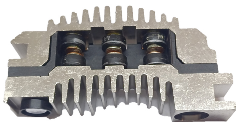
FA-DE-1119 Placa Delco 03472311; 7982718; DR3900 Austin, Opel, Chevrolet Kadett Å '91, Chevrolet Monza `82, Å '90 / Gmc Chevette CON DIODO AUXILIAR
