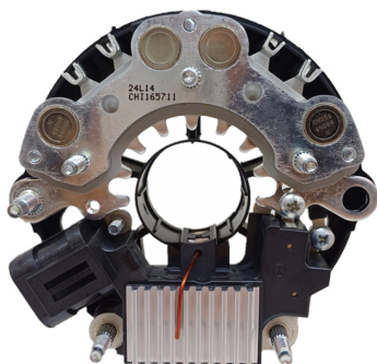
FA-H-1255 Placa Hitachi LR190-737, 23100 OW001 Nissan CON DIODO AUXILIAR
