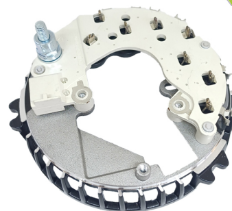
FA-F-1161 Placa Ford Ford F8RU-10A366-CA Ford Contor, Focus, Mercury, Cougar, Mystique CON DIODO AUXILIAR
