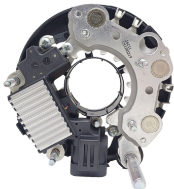
FA-H-1260 Placa Hitachi HITACHI LR170-505, LR170-505B Chevrolet Corsa diesel, Chevrolet Vectra diesel, Isuzu - diesel CON DIODO AUXILIAR
