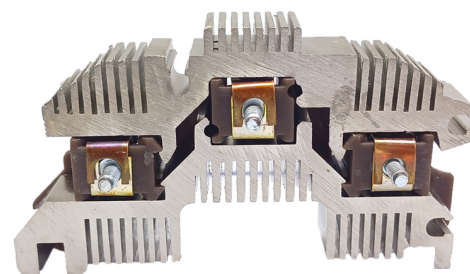
FA-DE-1118 Placa Delco 10467052; D3990 Chevrolet / Ford Mazda / Mitsubishi / Nissan; Gm Pick-up Van, Chevy Blazer, Gmc Suburban CON DIODO AUXILIAR
