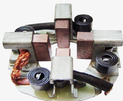
PCB-53 C/Carb. Mitsubishi Ford Van Diesel 8X24X18 SBE-351(146)
