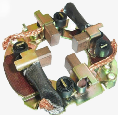
PCB-56 C/Carb. ArranqueMitsubishi Nissan Perkins Ford Dodge 8X24X18 SBE-351(159)
