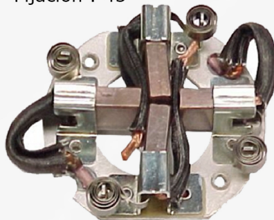
PCB-28 C/Carb. Arranque Indiel Motor Maxion Ford F-100 Diesel Ford Cargo LASX 15-27 M50R Fijacion : 73
