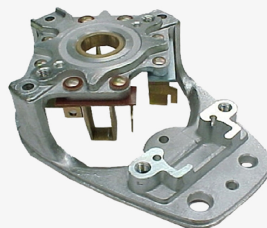
PCB-17 S/Carb. M/Benz Fiat Scania BPD Arranque FKB BSX 60
