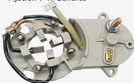
PCB-07 C/Carb. VW/Dodge 1.500 Gacel Arranque Tria
