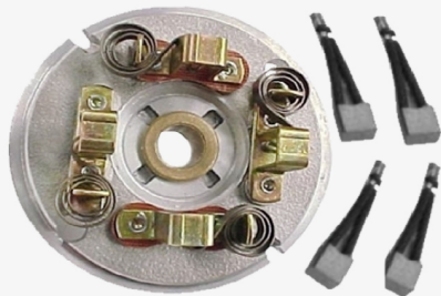
PCB-12-4 S/Carb. PCB-12-4/1 C/Carb. Peugeot 404-504 Fiat Dodge Arranque Garef USX-21-22
