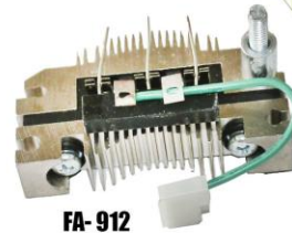
FA-912 P diodo M Marelli 63621501 Ducellier 593054 Lucas 21222124
