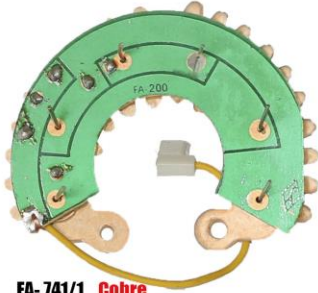
FA-741/1 Cobre M/Benz - Scania Deutz - Perkins -Fiat 45-70 Amp.
